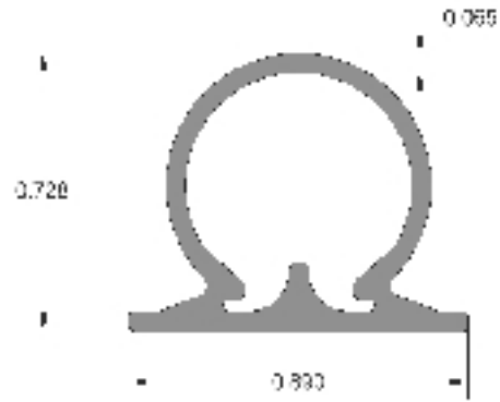
Figure 7 - Simple Drawing of Omega Profile
