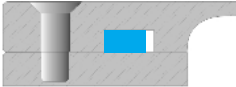
Figure 3 - Maximum Gland Fill Percentage
